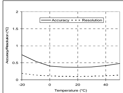
Plot A
